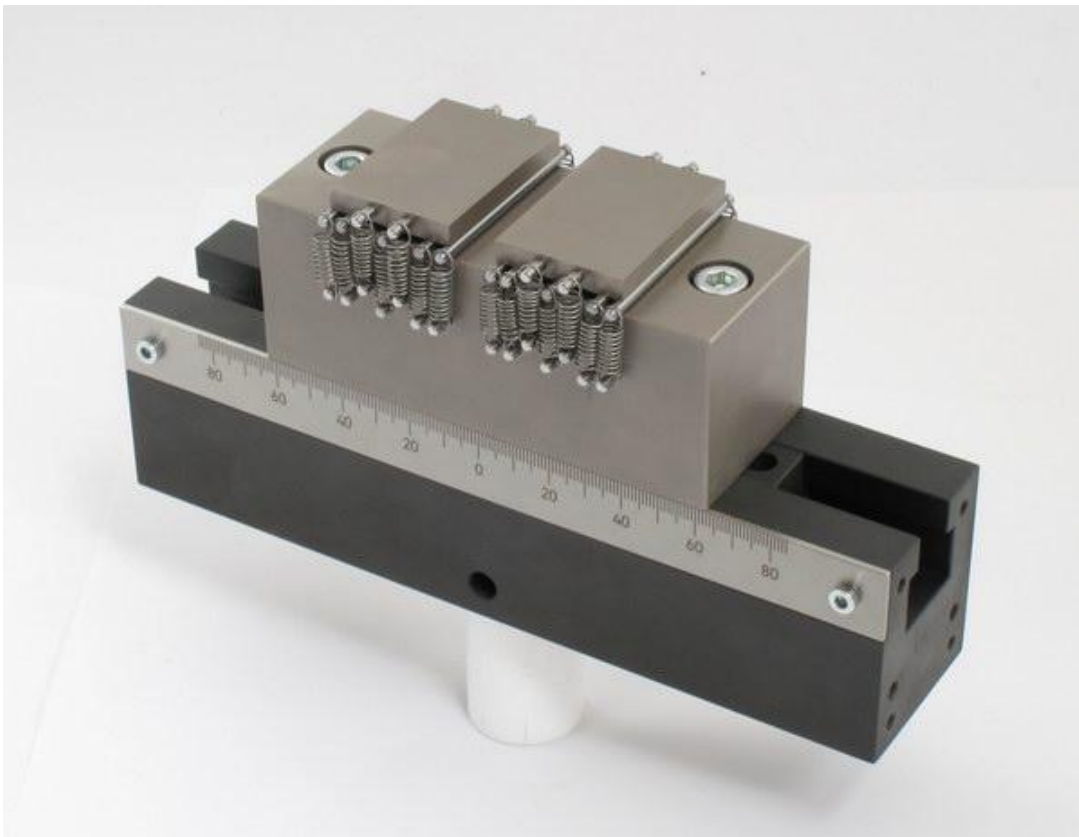
TH103-ASTMD234-Lower part with free moving slides
