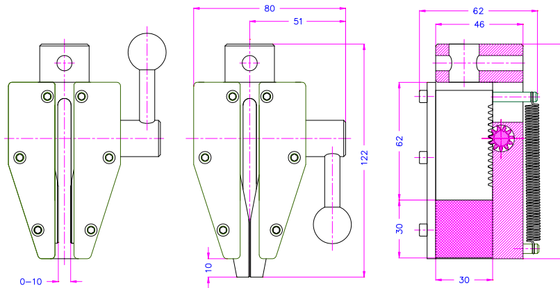
TH256
