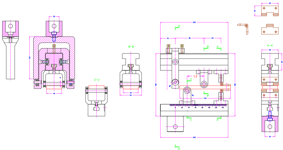
THS815-Af30 ASTM6671 mixed mode bending fixture interlaminar fracture toughness
