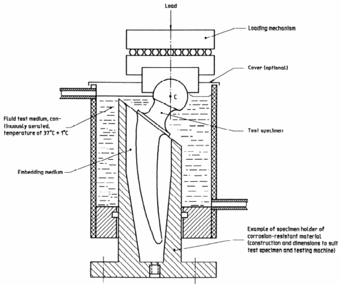
Figure 3 — General arrangement of specimen for testing
