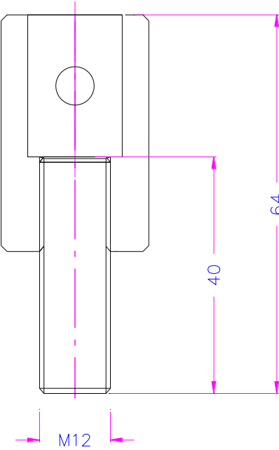
THS892-1665+M12x40
