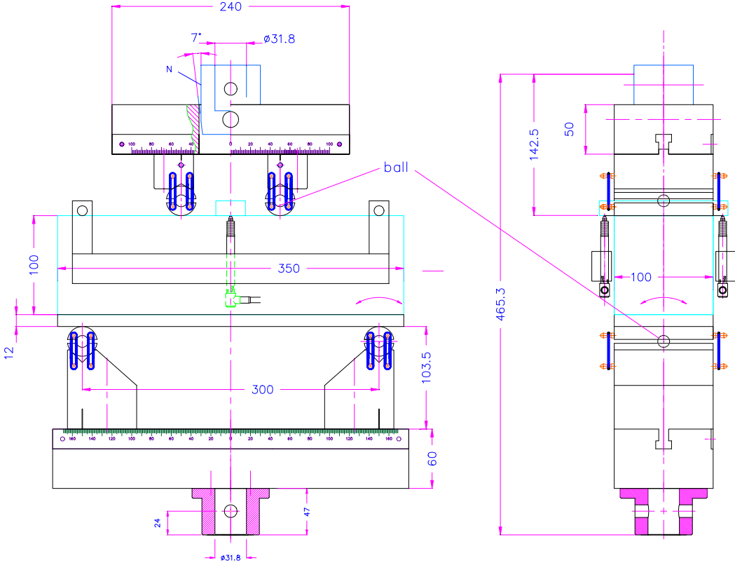
THS902-30 ASTM-C1399
